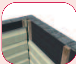
fig 9.1 Showing female component of 2-part corner trim being applied once cladding is finished
