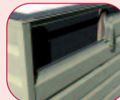
fig 10 Joint detail showing use of FC209 butt joint moulding
